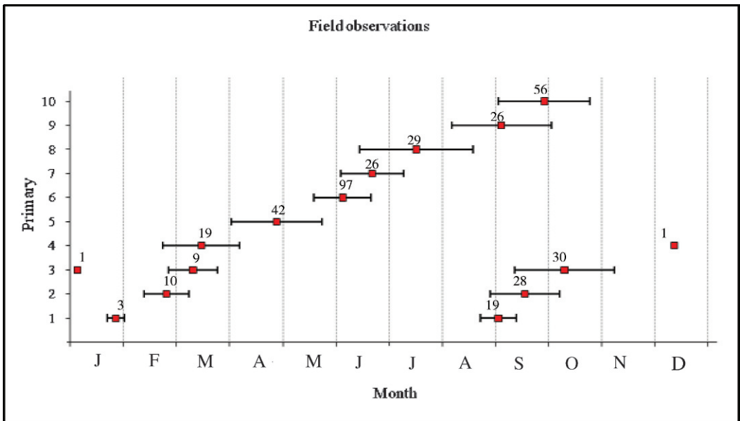
FIG. 2. Mean (± SE) feather drop date for Turkey Vultures by month based on field observations.
